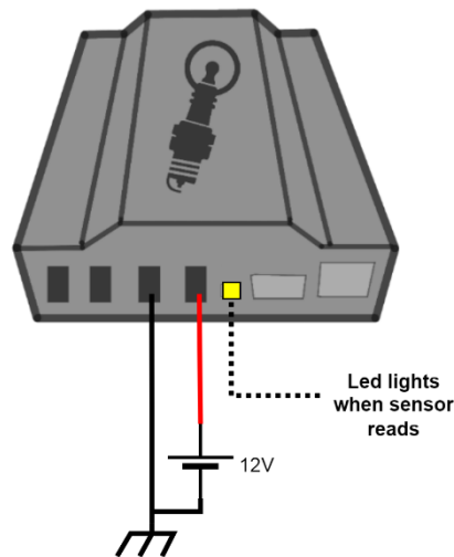
Figure 8: LED usage
