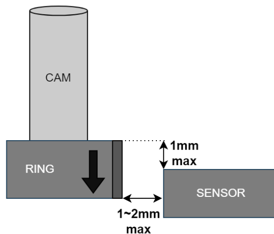
Figure 7: maximum distance and offset from sensor to ring
