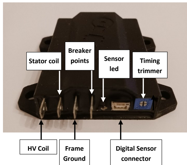
Figure 1: Front view
