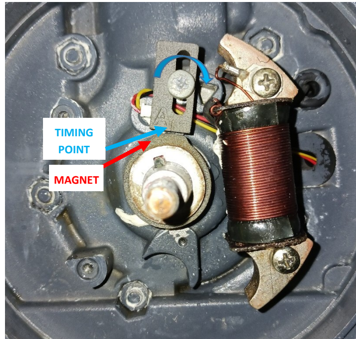
Figure 6: sensor mounting
